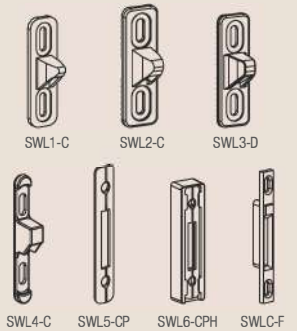
22 SLIDING WINDOW LATCH
