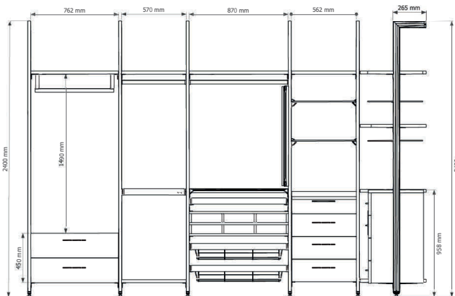
Aluminium Section
