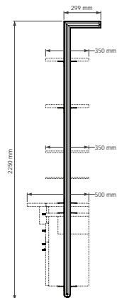
Adjustable Glass Shelf Support
