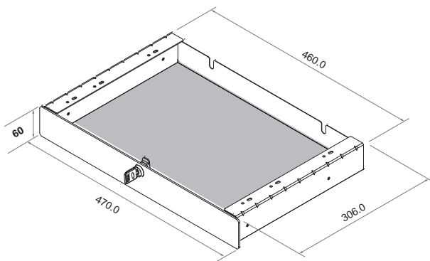
1 SDM-TM1 (With Felt Mat) / SD-TM1 (W/O Mat)
