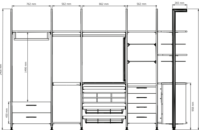
Aluminium Section
